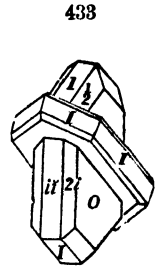
Bristol, Ct.
